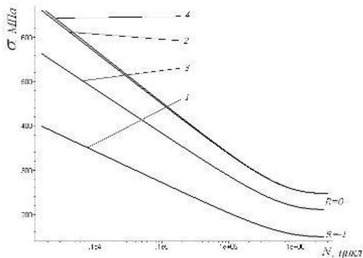
Figure 9 – Curves for samples of steel 17G1S [7, 15]:
